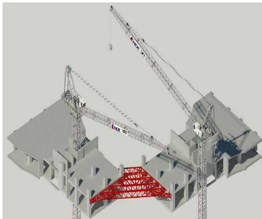
Installing the skybridge at floor 49th
