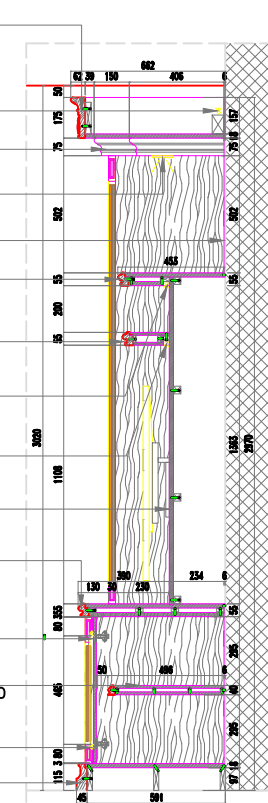
SECTION 1 SCALE 1:16
