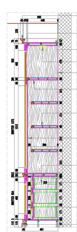
SECTION 2 SCALE 1:16
